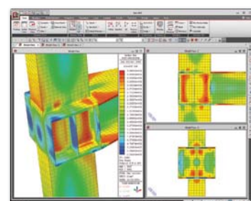
[ Detail Analysis ]
