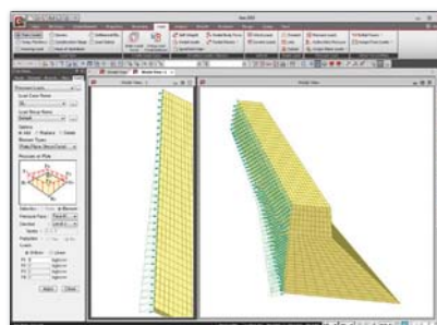
[Pressure Load Generation]
