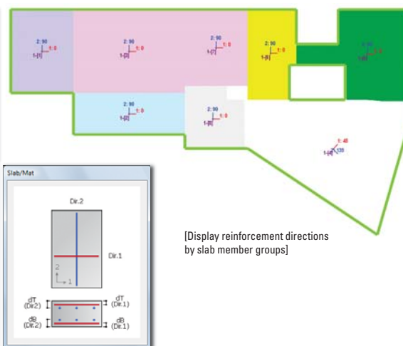
[Define reinforcement directions]
