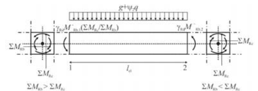
[Capacity design shear forces on beams]
